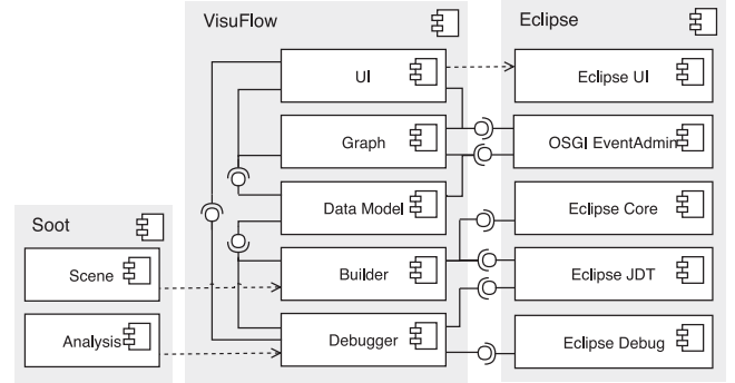
Fig. 5. Component diagram of VISUFLOW.
