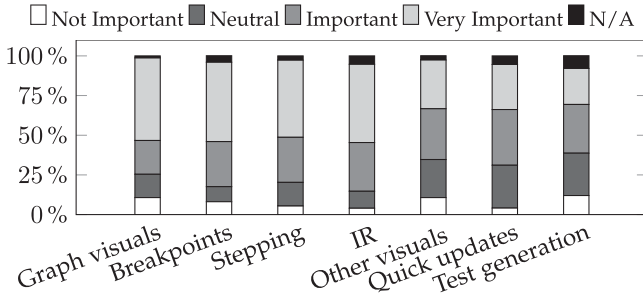
Fig. 4. Ranking the importance of features for debugging static analysis. IR is “Intermediate representation” (Q26).
