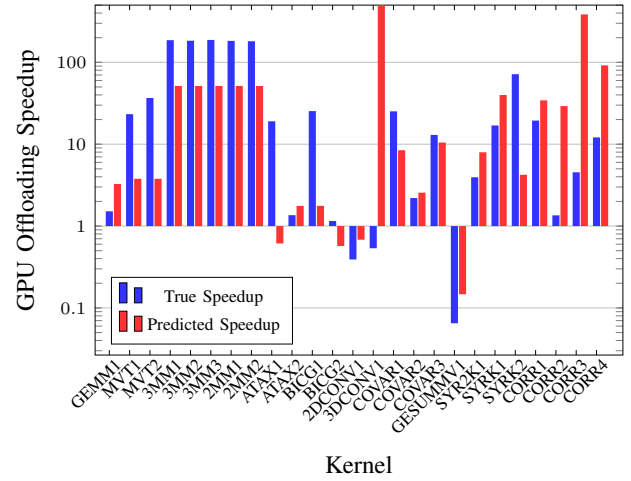
Figure 6: Actual versus predicted GPU offloading speedup for test kernel execution mode versus a host using 4 threads.
