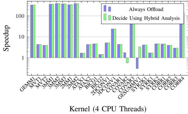
Figure 8: Speedup achieved by always offloading to GPU versus offloading when determined profitable by the analytical hybrid decision model. Benchmarks executed in Benchmark mode.
