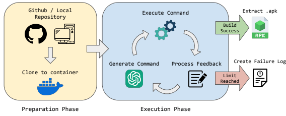
Fig. 1. The high-level workflow of BuildDroid.
